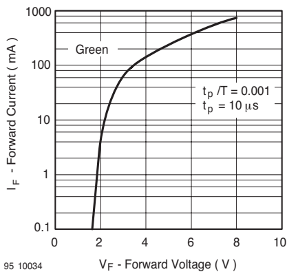
Figure 20. Forward Current vs. Forward Voltage
