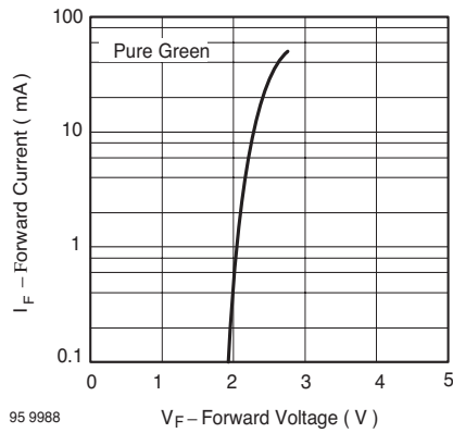
Figure 25. Forward Current vs. Forward Voltage
