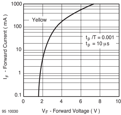
Figure 15. Forward Current vs. Forward Voltage
