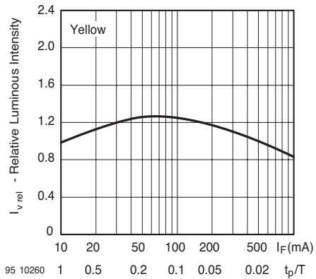
Figure 17. Rel. Lumin. Intensity vs. Forw. Current/Duty Cycle
