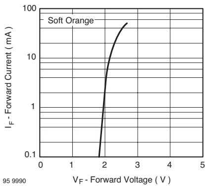
Figure 10. Forward Current vs. Forward Voltage
