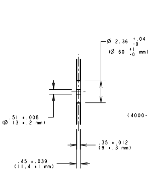
REEL SPECIFICATION NO SCALE
