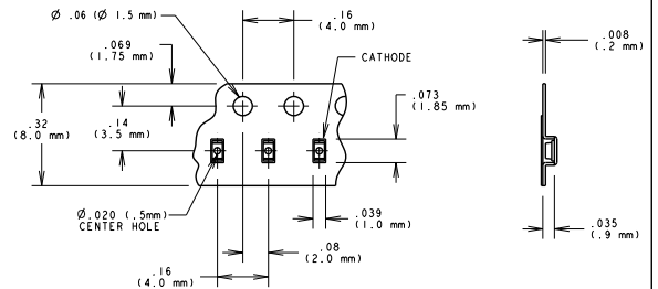
TAPE & REEL SPECIFICATION NO SCALE
