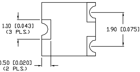
TAPE SPEC DETAIL
