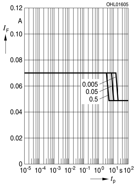
Zulässige Impulsbelastbarkeit I_F = f(t_p) Permissible Pulse Handling Capability Duty cycle D = parameter, T_A = 25\text{ °C} amber (3 Chips on)
