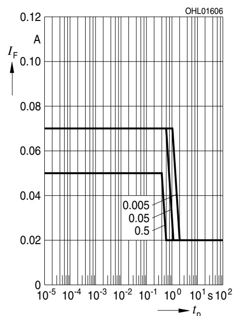
Zulässige Impulsbelastbarkeit I_F = f(t_p) Permissible Pulse Handling Capability Duty cycle D = parameter, T_A = 85\text{ °C} amber (3 Chips on)
