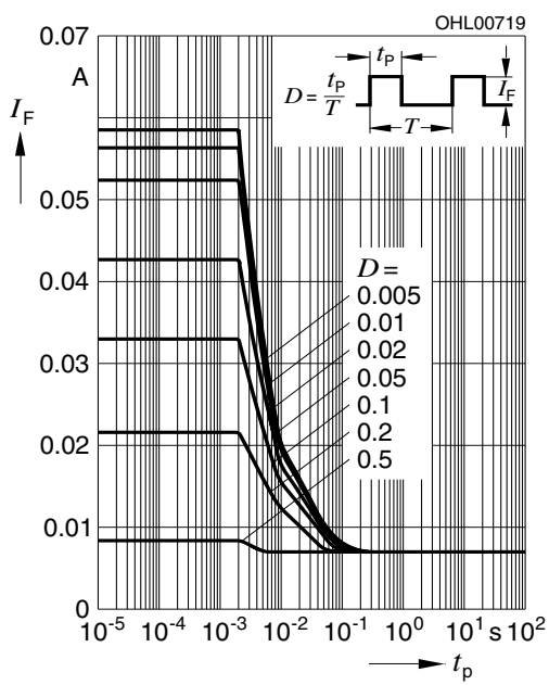
Zulässige Impulsbelastbarkeit I_F = f(t_p) Permissible Pulse Handling Capability Duty cycle D = parameter, T_A = 85\text{ °C} blue (3 Chips on)
