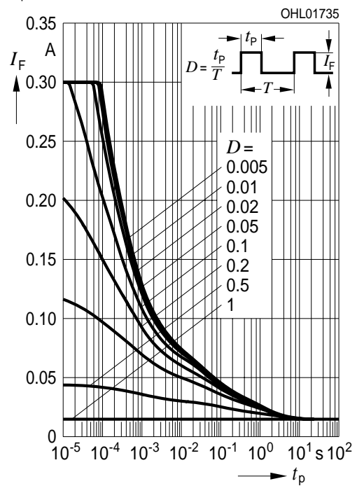
Zulässige Impulsbelastbarkeit Permissible Pulse Handling Capability Duty cycle D = \text{parameter} , T_A = 85\text{ °C} I_F = f(t_p) ; true green (3 Chips on)
