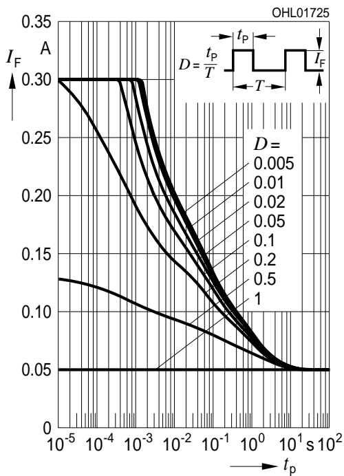
Zulässige Impulsbelastbarkeit Permissible Pulse Handling Capability Duty cycle D = \text{parameter} , T_A = 85\text{ °C} I_F = f(t_p) ; true green (1 Chip on)
