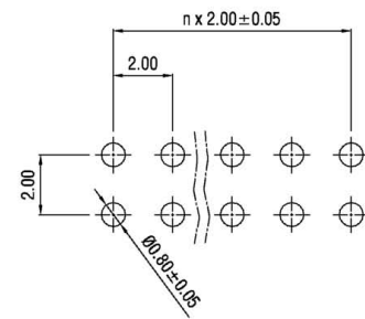
PCB Layouts
