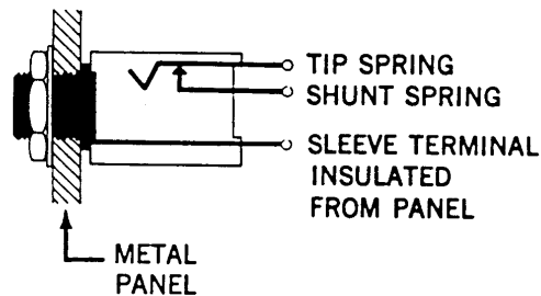
INSULATED MOUNTING
