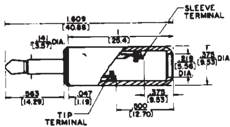
No. 740 Screw Terminals
