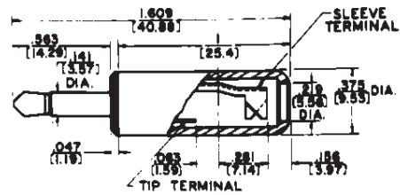
No. 750 Clamp-Lug Terminals
