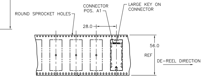
TAPE & REEL PACKAGING PER EIA 481-3 SCALE NONE
