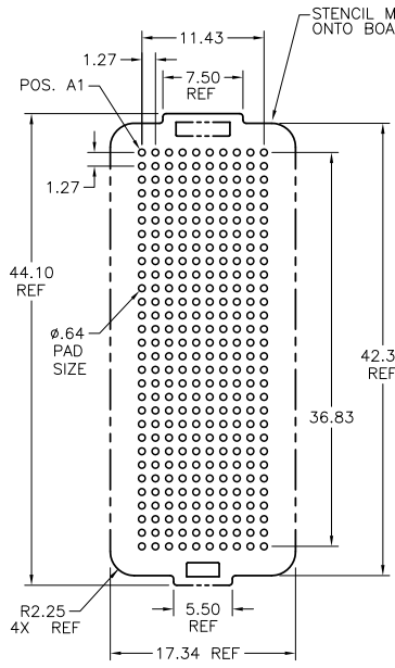
BOARD PATTERN
