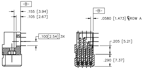
SECTION U-U SECTION X-X
