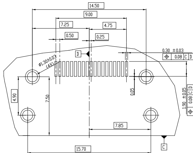
RECOMMENDED PCB PATTERN LAYOUT (t=1.6mm)
