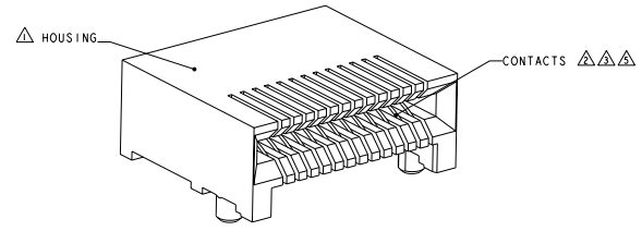
26 POSITION RECEPTACLE SCALE 9:1
