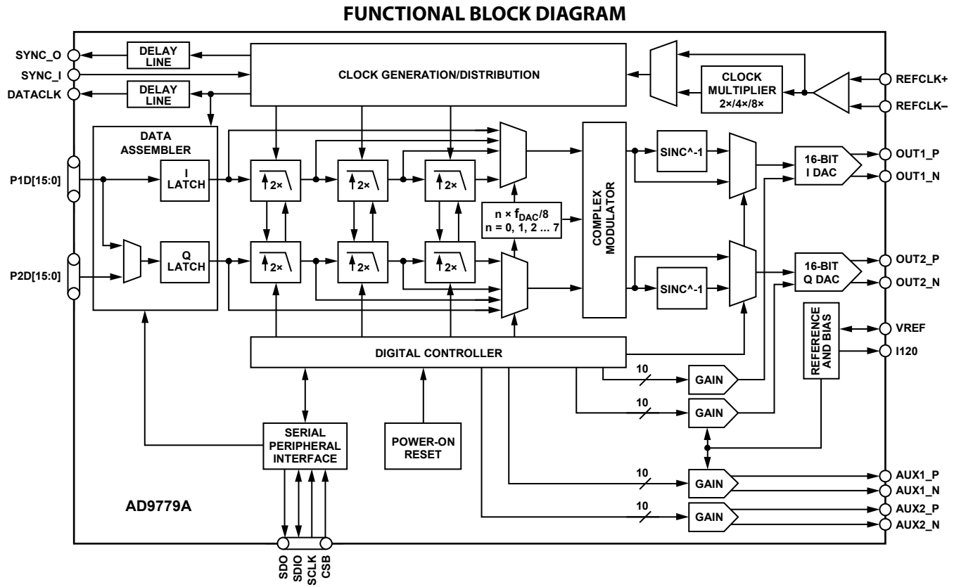
Figure 2. AD9779A Functional Block Diagram
