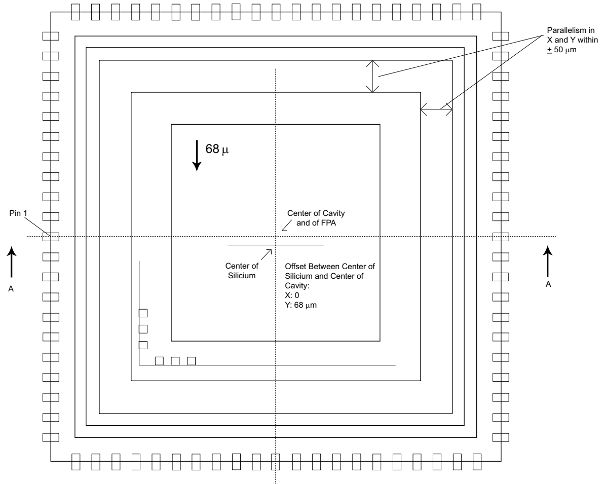
Figure 14. Die Alignment
