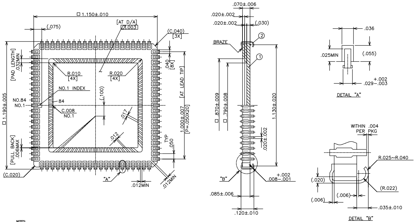
Figure 13. STAR250 Package Dimensions
