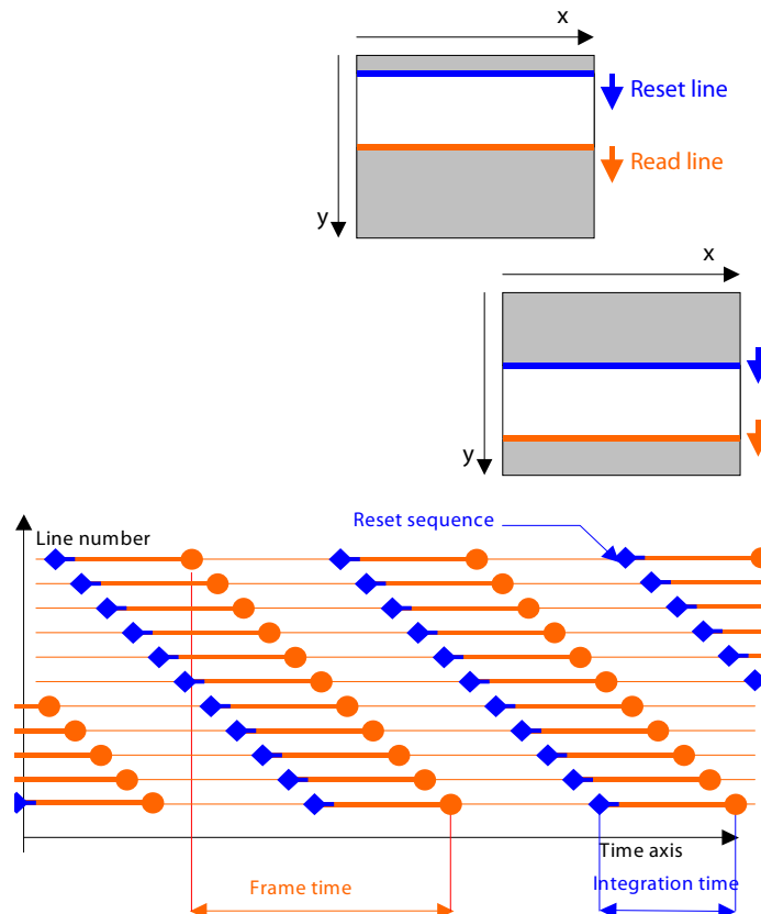
Figure 9. Electronic Shutter
