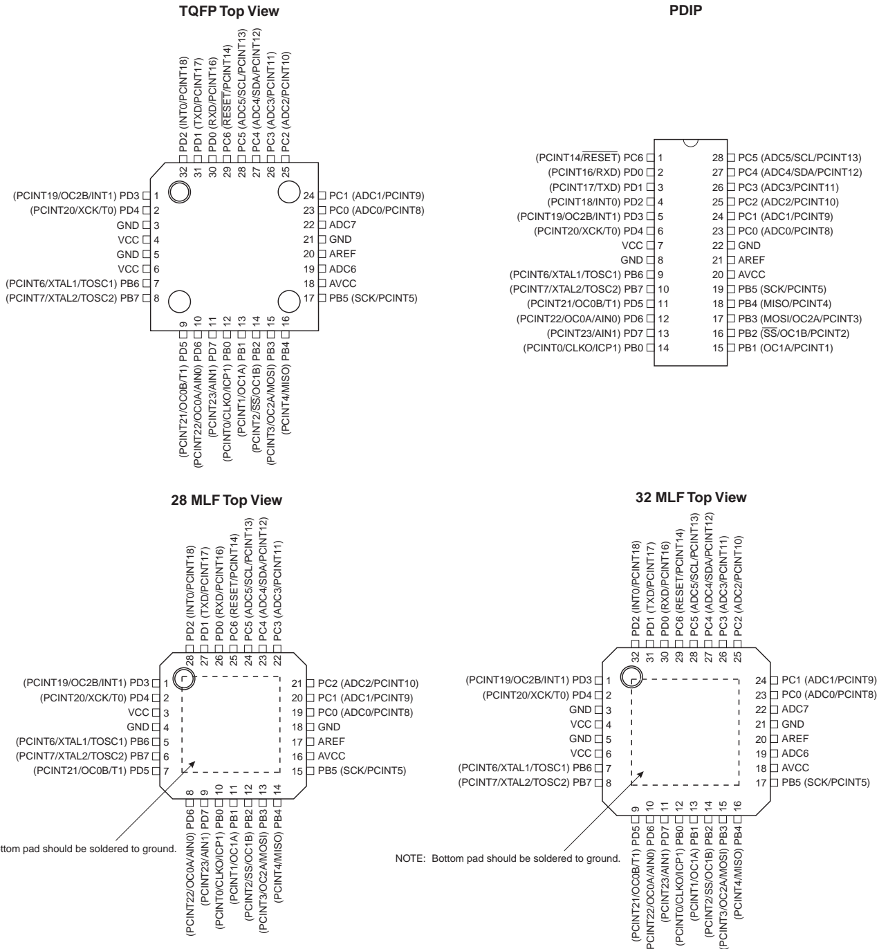
Figure 1-1. Pinout ATmega48/88/1682545LS
