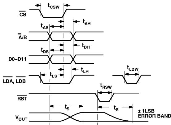
Timing Diagram
