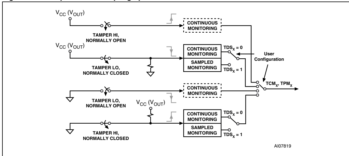
Figure 16. Tamper detect sampling options
