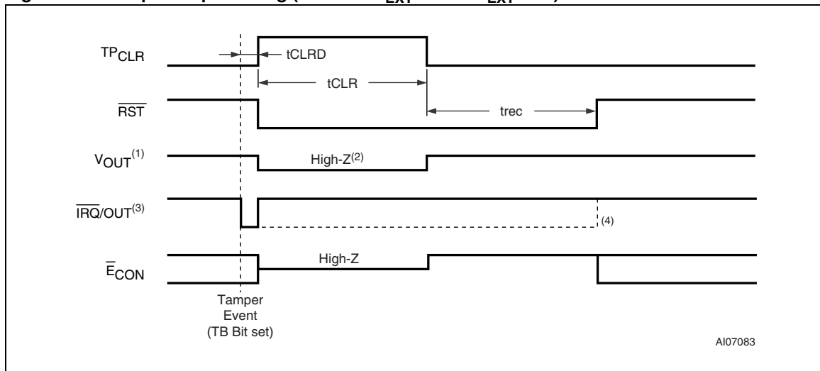
Figure 18. Tamper output timing (with CLR1_{EXT} or CLR2_{EXT} = '1' )
