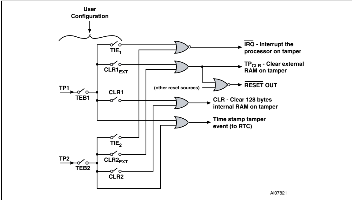
Figure 15. Basic tamper detect options
