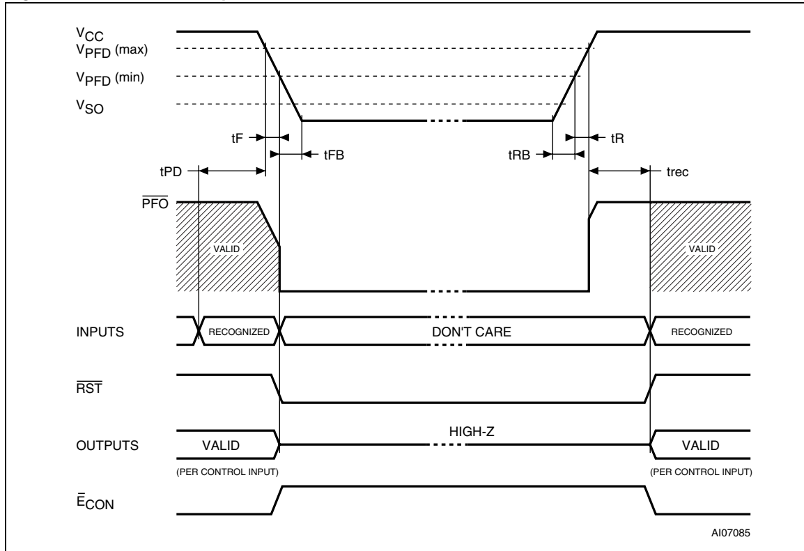
Figure 27. Power down/up mode AC waveforms
