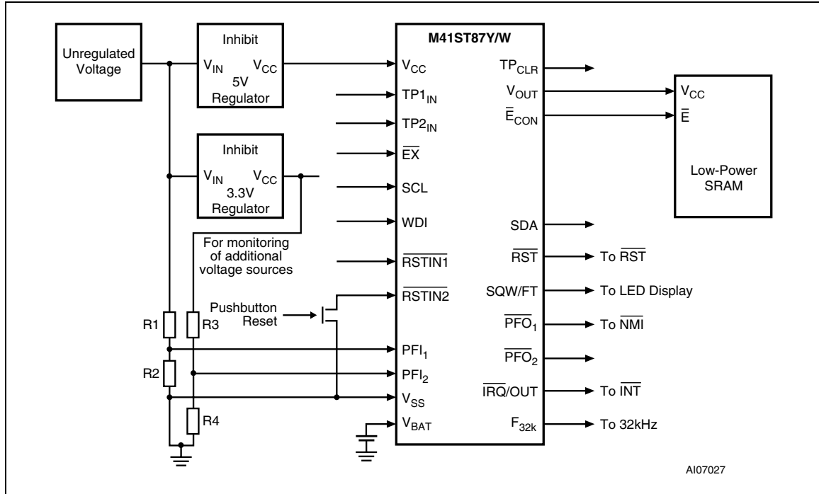
Figure 4. Hardware hookup
