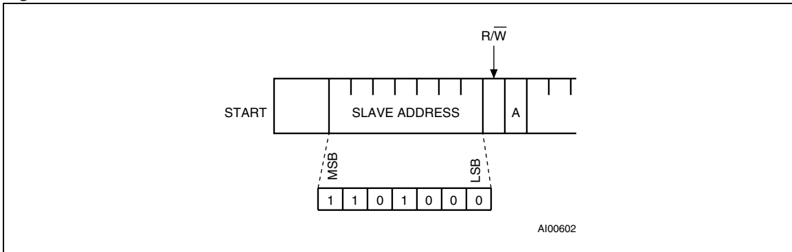
Figure 9. READ mode sequence
