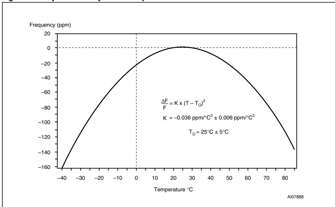
Figure 21. Crystal accuracy across temperature
