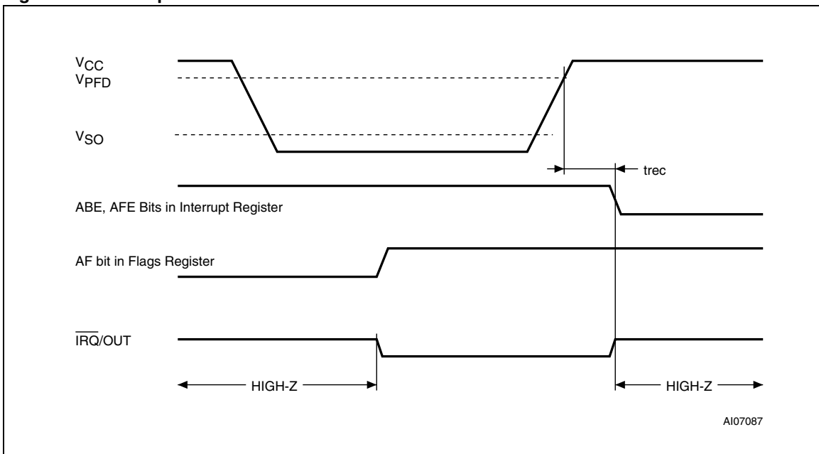
Figure 24. Backup mode alarm waveform
