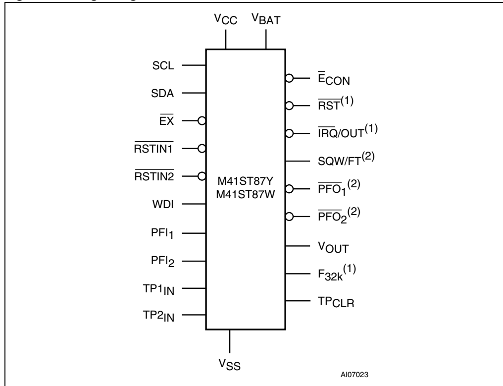
Figure 1. Logic diagram
