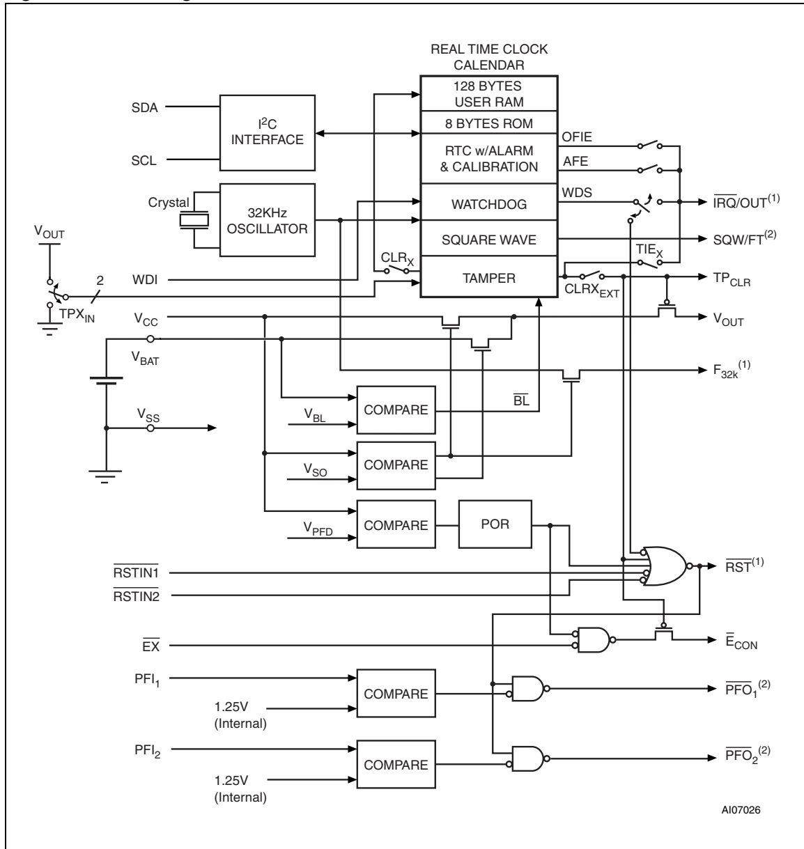
Figure 3. Block diagram
