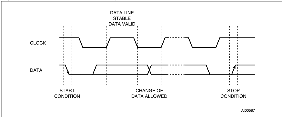
Figure 6. Acknowledgement sequence
