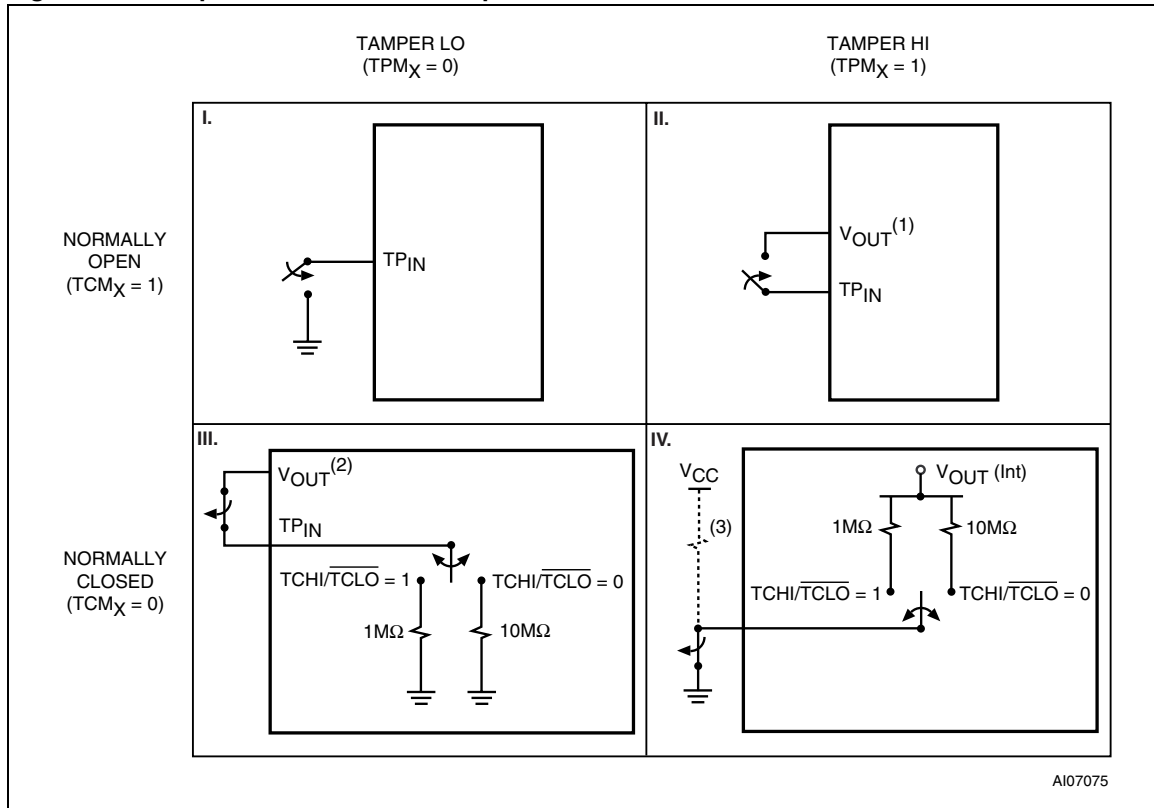
Figure 13. Tamper detect connection options
