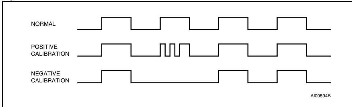
Figure 22. Calibration waveform
