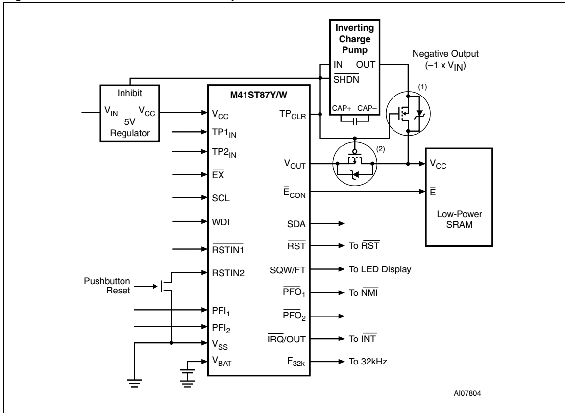
Figure 19. RAM clear hardware hookup
