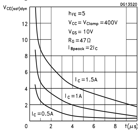
Figure 16: Inductive Load Enlargement FBSOA Circuit
