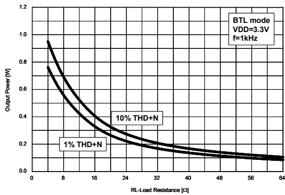
Figure 39. Output Power vs. Load Resistance
