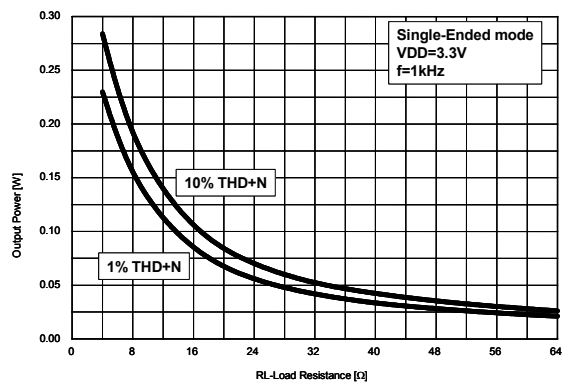
Figure 42. Output Power vs. Load Resistance
