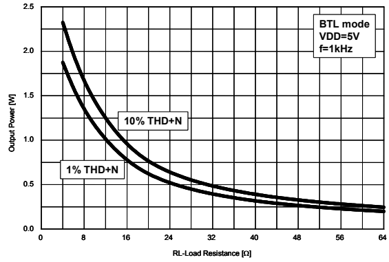
Figure 38. Output Power vs. Load Resistance
