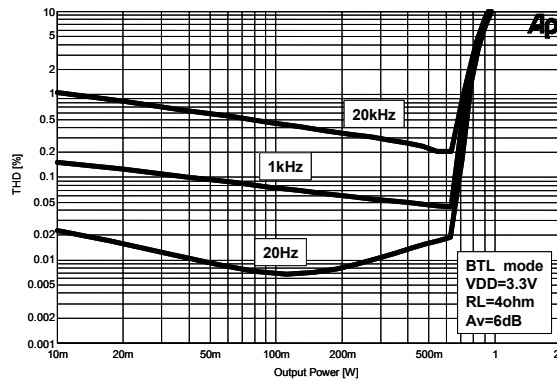
Figure 3. THD+N vs. Output Power
