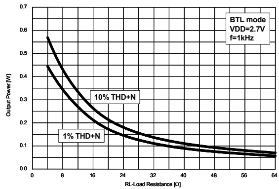
Figure 40. Output Power vs. Load Resistance
