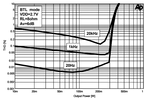
Figure 6. THD+N vs. Output Power
