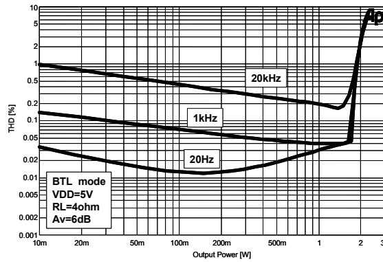
Figure 1. THD+N vs. Output Power
