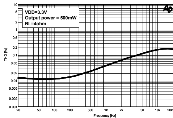
Figure 12. THD+N vs. Frequency
