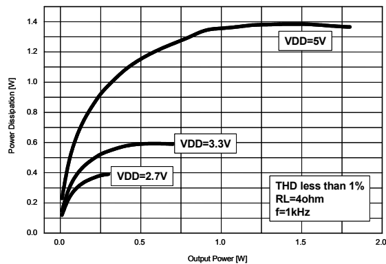
Figure 35. Power Dissipation vs. Output Power
