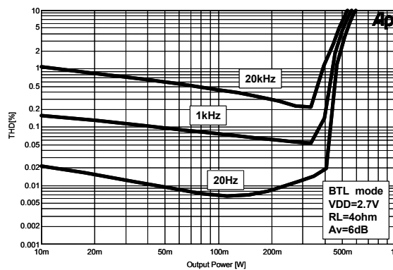
Figure 5. THD+N vs. Output Power
