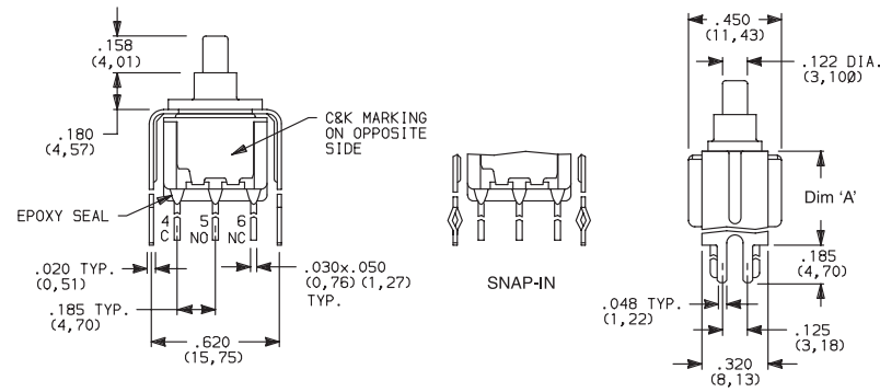
8221SD3_GE DPDT
