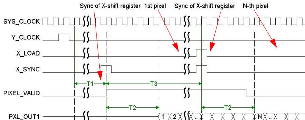
Figure 24. Pixel Output
