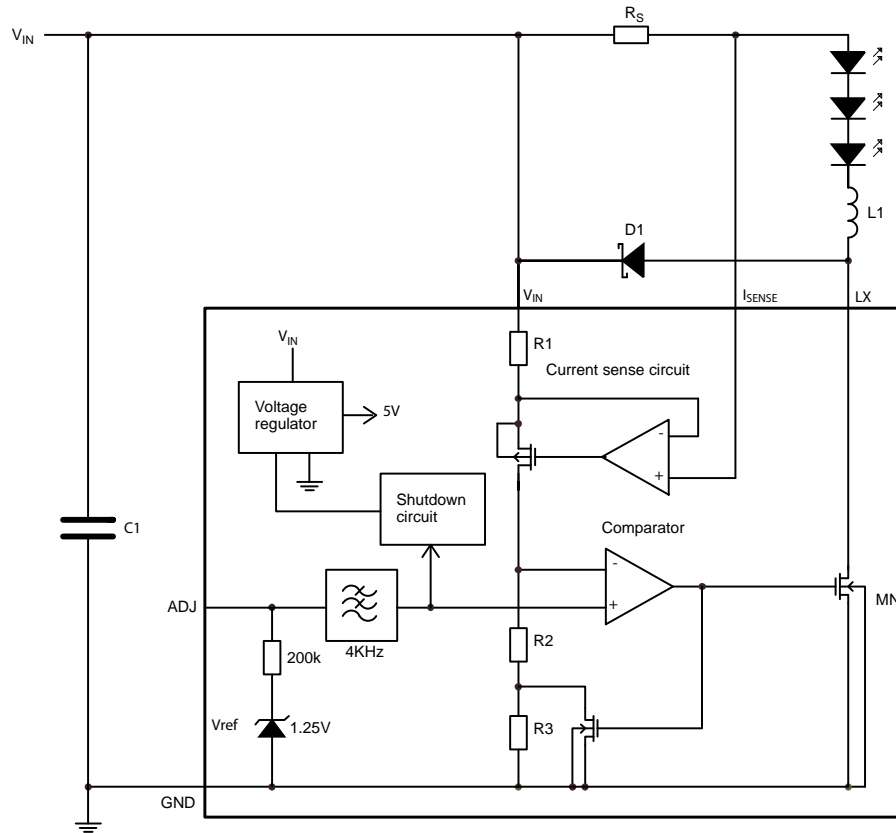
Figure 1. Block diagram – Pin Connection for TSOT Package
