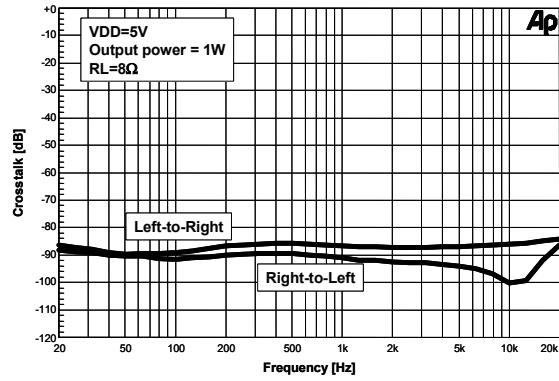
Figure 20. Crosstalk vs. Frequency
