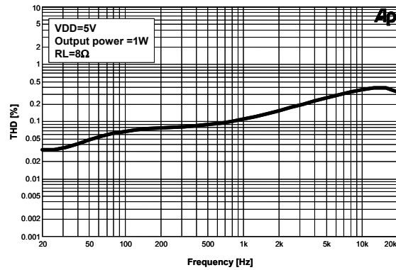
Figure 40. THD+N vs. Frequency
