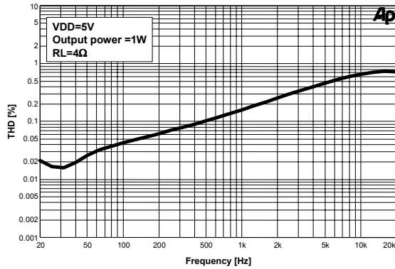
Figure 7. THD+N vs. Frequency
