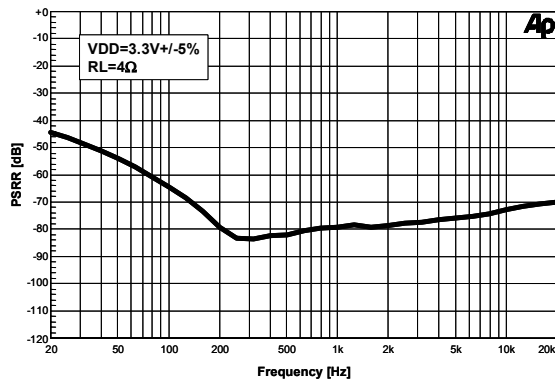
Figure 15. PSRR vs. Frequency
