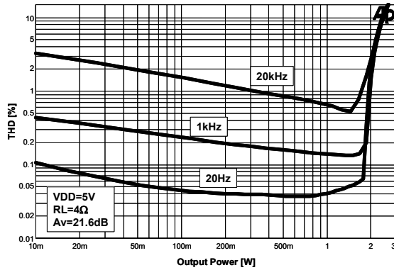
Figure 33. THD+N vs. Output Power
