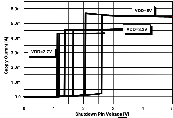
Figure 22. Supply Current vs. SD Voltage
