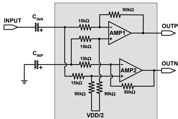
Case (B) : AC Coupling to Ground
