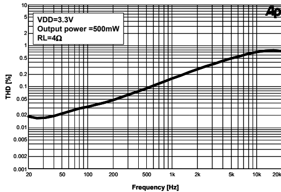
Figure 9. THD+N vs. Frequency
