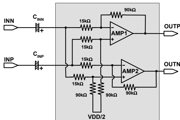
Figure 1. Configuration of Power Amplifier
