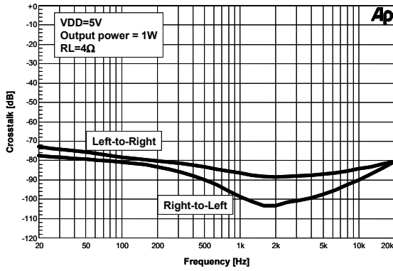
Figure 19. Crosstalk vs. Frequency
