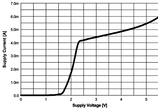
Figure 21. Supply Current vs. Supply Voltage
