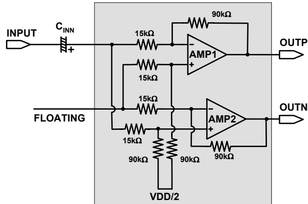
Case (A) : Residual Input Pin Floating
