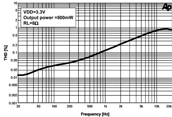
Figure 10. THD+N vs. Frequency
