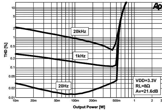
Figure 36. THD+N vs. Output Power
