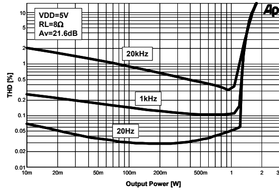
Figure 34. THD+N vs. Output Power
