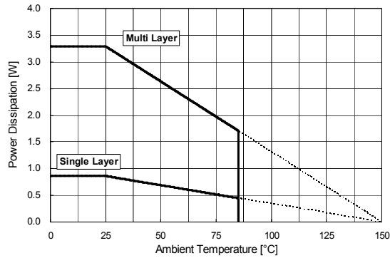
Figure 45. Power Derating Curve
