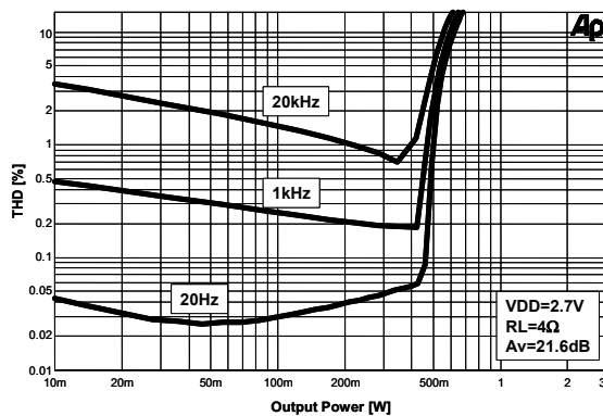
Figure 37. THD+N vs. Output Power
