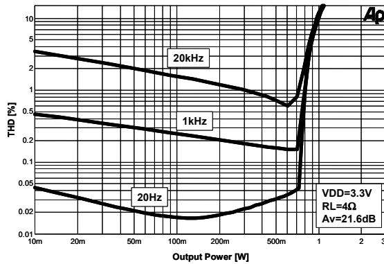
Figure 35. THD+N vs. Output Power
