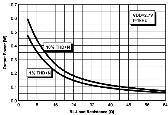
Figure 29. Output Power vs. Output Load
