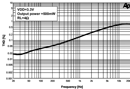
Figure 41. THD+N vs. Frequency
