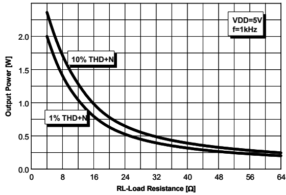
Figure 27. Output Power vs. Output Load
