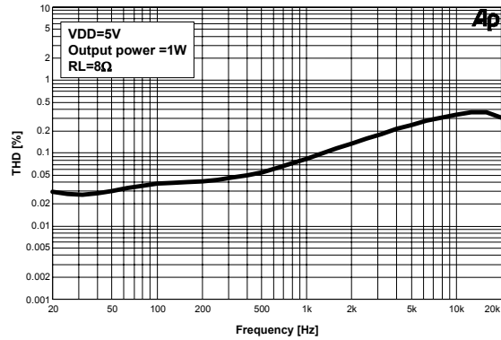
Figure 8. THD+N vs. Frequency
