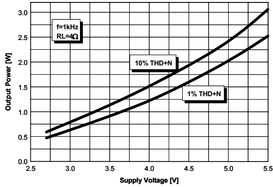
Figure 25. Output Power vs. Supply Voltage
