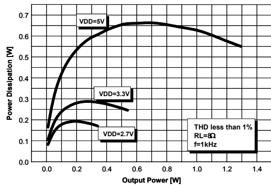
Figure 24. Power Dissipation vs. Output Power
