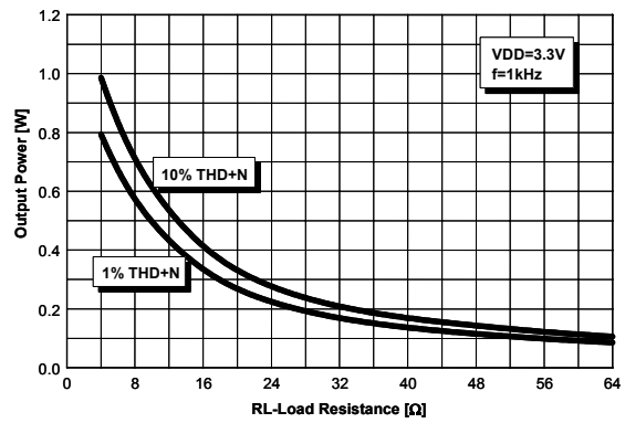
Figure 28. Output Power vs. Output Load
