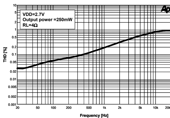
Figure 43. THD+N vs. Frequency
