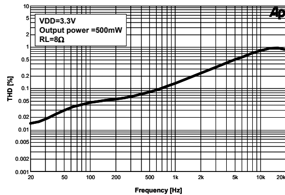
Figure 42. THD+N vs. Frequency
