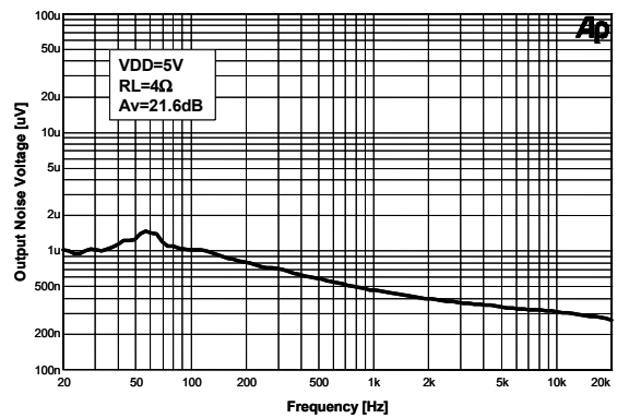
Figure 30. Output Noise Voltage vs. Frequency
