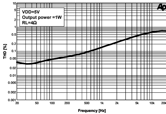
Figure 39. THD+N vs. Frequency
