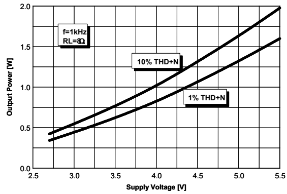
Figure 26. Output Power vs. Supply Voltage
