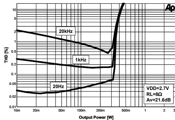
Figure 38. THD+N vs. Output Power
