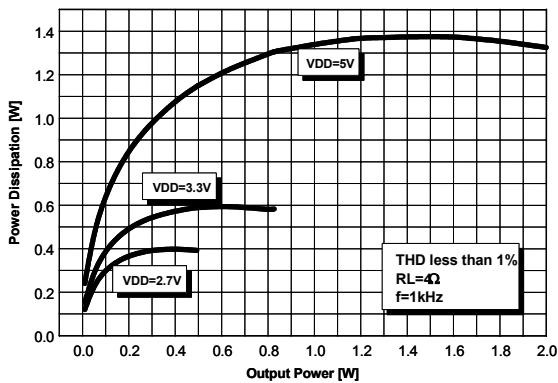
Figure 23. Power Dissipation vs. Output Power
