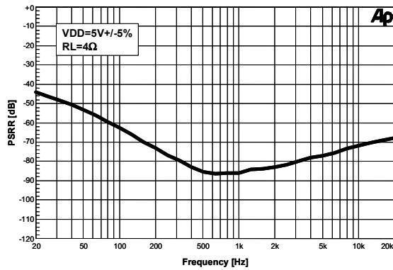
Figure 13. PSRR vs. Frequency
