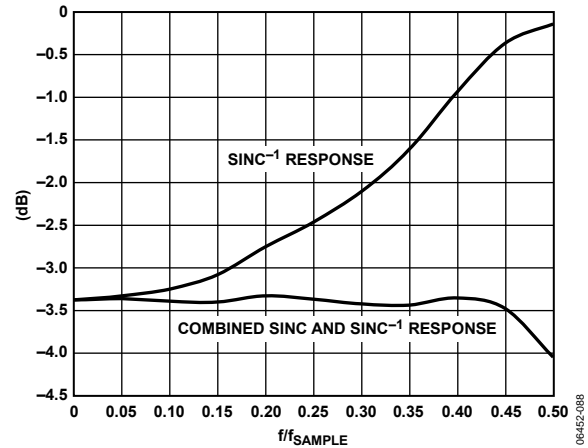
Figure 71. Transfer Function of Inverse Sinc Filter with the DAC \sin(x)/x Output
