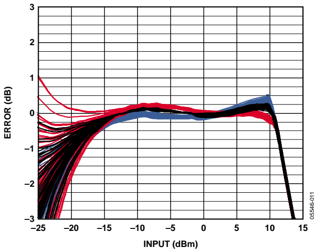
Figure 11. Temperature Drift Distributions for 55 Devices at -40^{\circ}\text{C} , +25^{\circ}\text{C} , and +85^{\circ}\text{C} vs. +25^{\circ}\text{C} Linear Reference, Frequency 900 MHz, Supply 5.0 V
