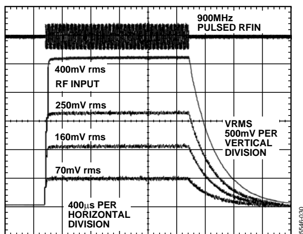
Figure 30. Output Response to Modulated Pulse Input for Various RF Input Levels, Supply 3 V, Modulation Frequency 900 MHz, 0.01 \mu F Filter Capacitor
