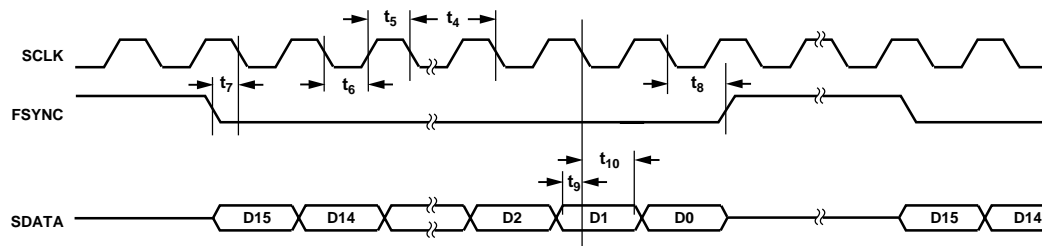
Figure 3. Serial Timing
