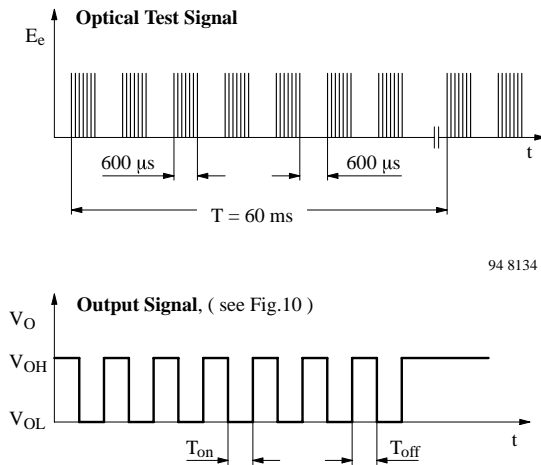
Figure 8. Output Function
