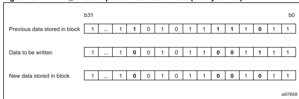
Figure 13. WRITE_BLOCK update in standard mode (binary format)
