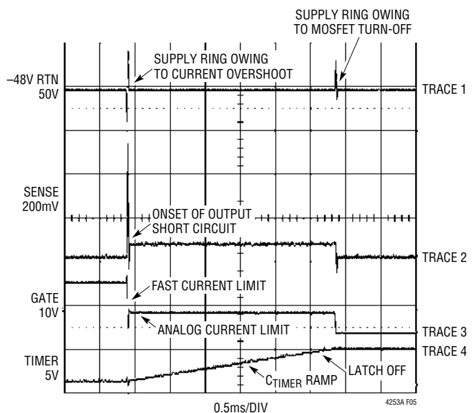
Figure 5. Output Short-Circuit Behavior of LTC4253A-ADJ
