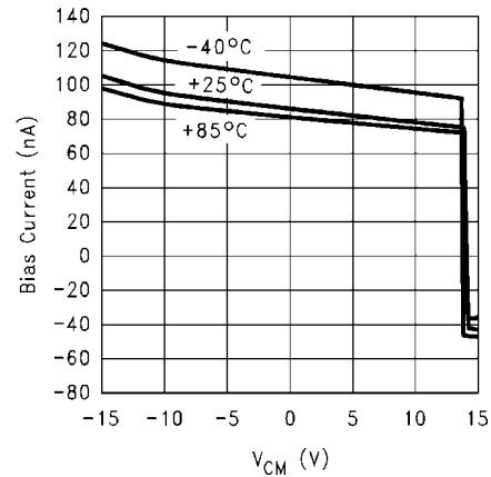
Non-Inverting Input Bias Current vs. Common Mode Voltage V_S = \pm 15V
