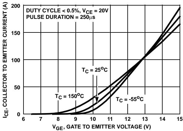
FIGURE 13. TRANSFER CHARACTERISTIC
