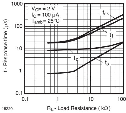
Figure 8. Response Time vs. Load Resistance
