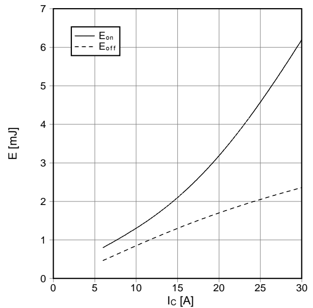
Schaltverluste IGBT-Wechselr. (typisch) switching losses IGBT-inverter (typical) E_{on} = f(I_c) , E_{off} = f(I_c) V_{GE} = \pm 15\text{ V} , R_{Gon} = 75\ \Omega , R_{Goff} = 75\ \Omega , V_{CE} = 600\text{ V} , T_{vj} = 125^\circ\text{C}
