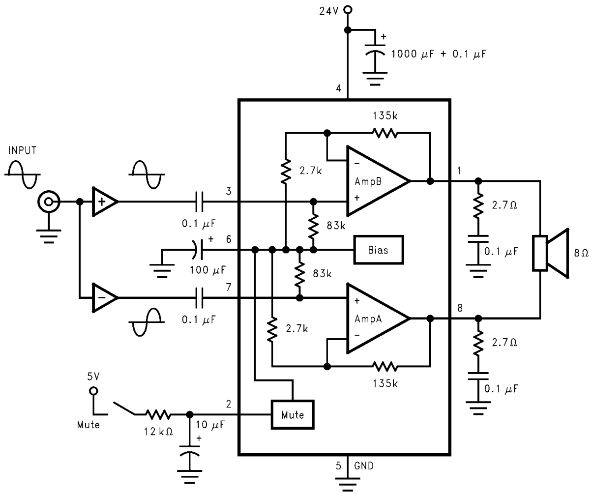
FIGURE 4. Bridge-Mode Application
