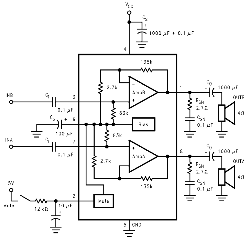
FIGURE 1. Typical Audio Amplifier Application Circuit
