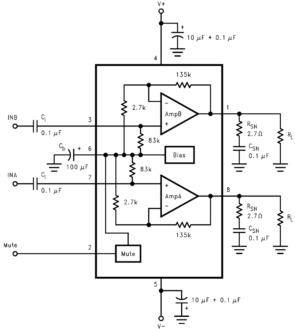
FIGURE 2. Test Circuit
