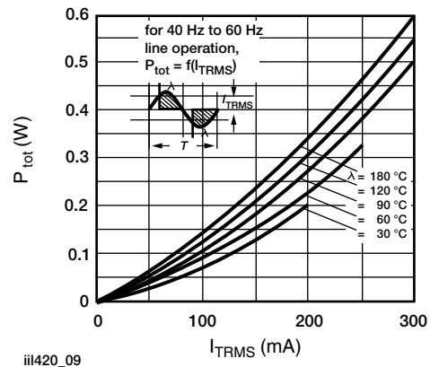
Fig. 9 - Power Dissipation
