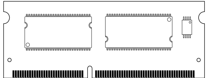
Figure 1: 144-Pin SODIMM (MO-190)
