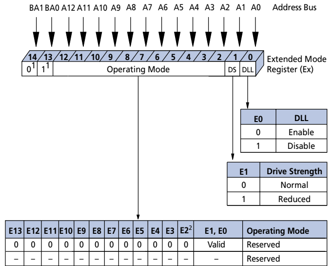
Figure 6: Extended Mode Register Definition Diagram
