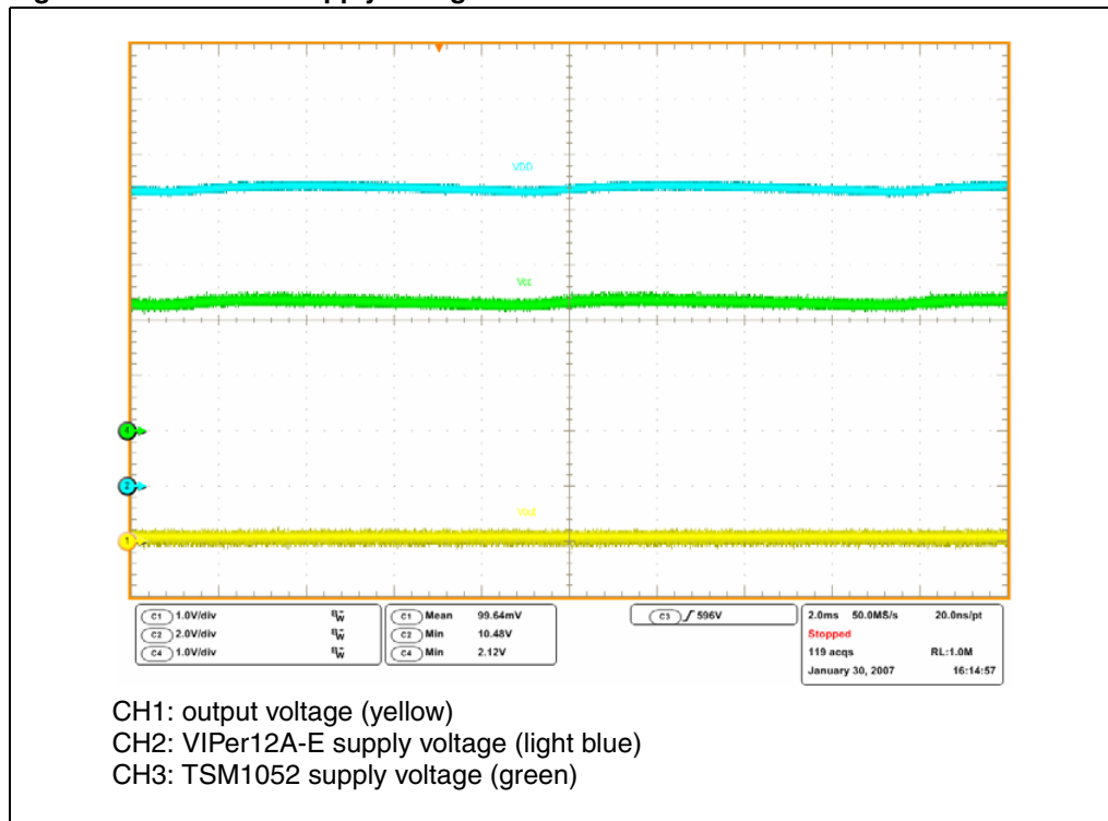
Figure 6. Minimum supply voltages
