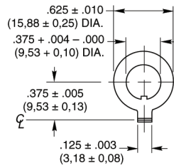
Non-Turn Washer
