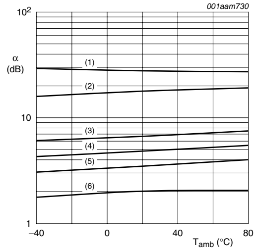
V_{CC} = 0.75 \text{ V}; f = 3000 \text{ MHz}. (1) V_{ctrl} = 0 \text{ V} (2) V_{ctrl} = 1 \text{ V} (3) V_{ctrl} = 2 \text{ V} (4) V_{ctrl} = 3 \text{ V} (5) V_{ctrl} = 5 \text{ V} (6) V_{ctrl} = 10 \text{ V}
