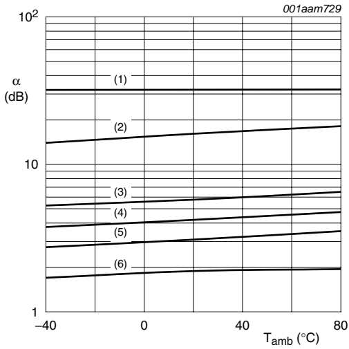
V_{CC} = 0.75 \text{ V}; f = 2000 \text{ MHz}. (1) V_{ctrl} = 0 \text{ V} (2) V_{ctrl} = 1 \text{ V} (3) V_{ctrl} = 2 \text{ V} (4) V_{ctrl} = 3 \text{ V} (5) V_{ctrl} = 5 \text{ V} (6) V_{ctrl} = 10 \text{ V}
