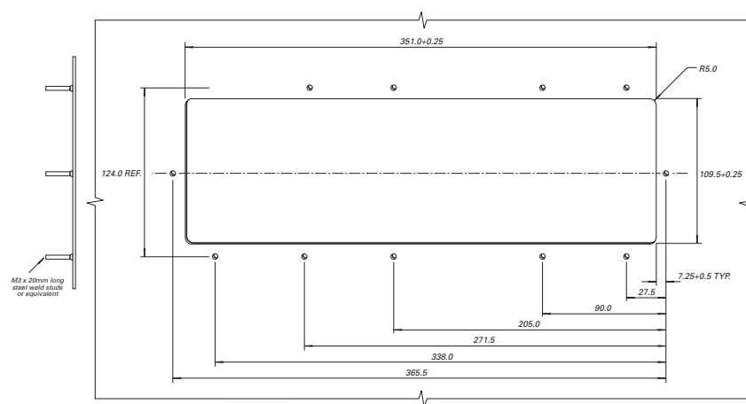
View showing rear of panel with dimensions of stud positions and panel cut out details All dimensions in mm.
