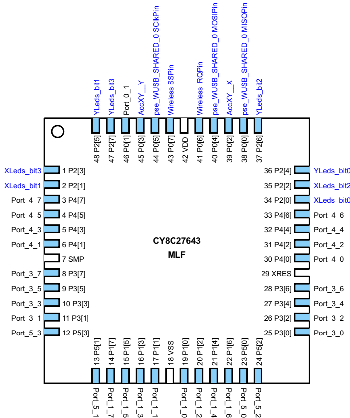
Figure 8-1. CY3209WUSBTiltSlave Pinouts
