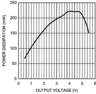
Power Dissipation vs Output Power V_{DD} = 4.2V, R_L = 2\mu F + 30\Omega, f = 1kHz
