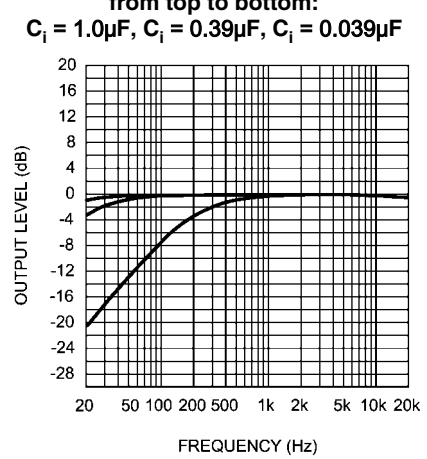
Frequency Response vs Input Capacitor Size R_L = 8\Omega from top to bottom: C_i = 1.0\mu F, C_i = 0.39\mu F, C_i = 0.039\mu F
