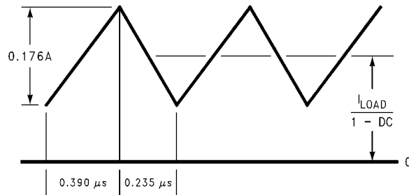
FIGURE 3. 10μH Inductor Current 5V - 12V Boost (LM4961X)
