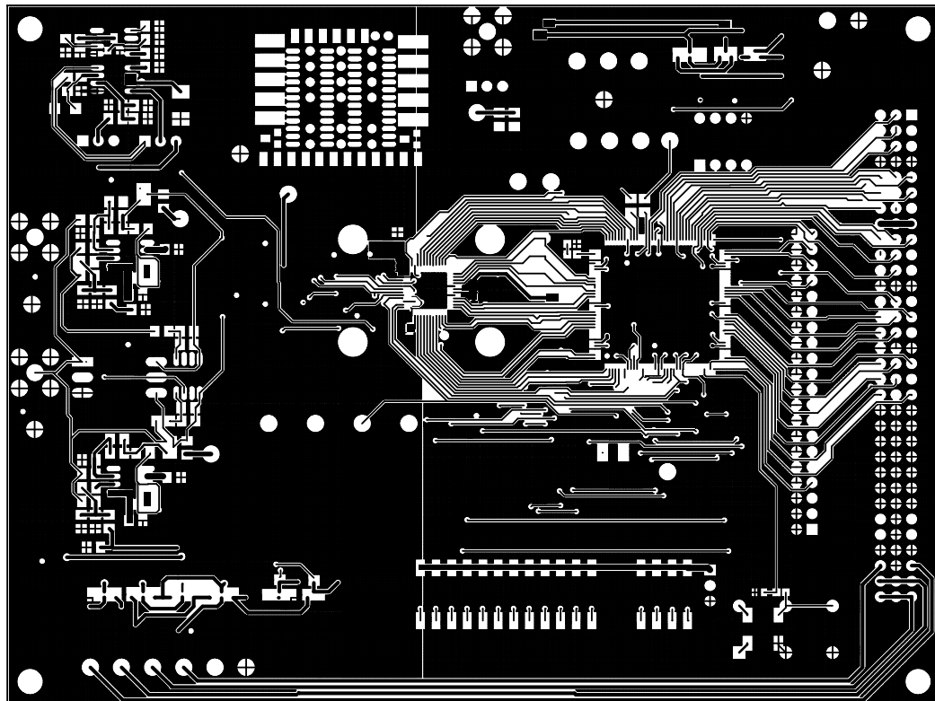
Figure 6. Top Layer
