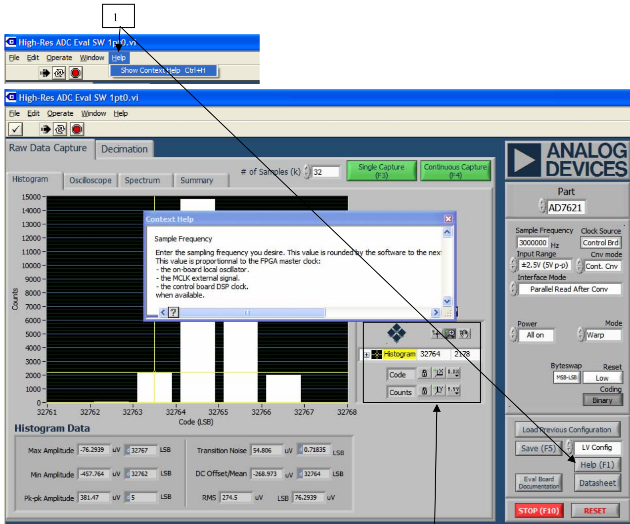
Figure 12. Context Help
