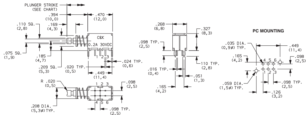
PN21SBSA03QE DPDT
