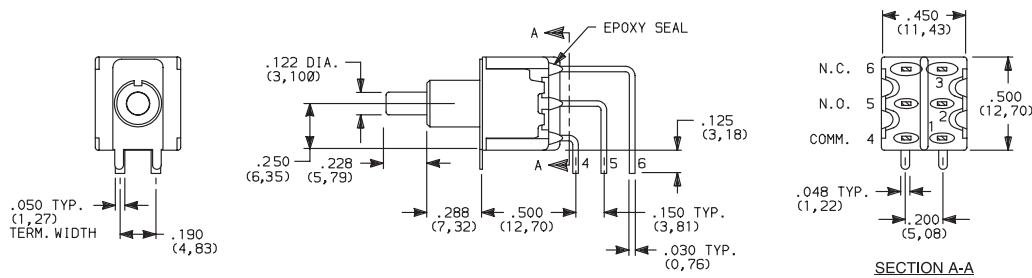
8221SD9AV2GE DPDT
