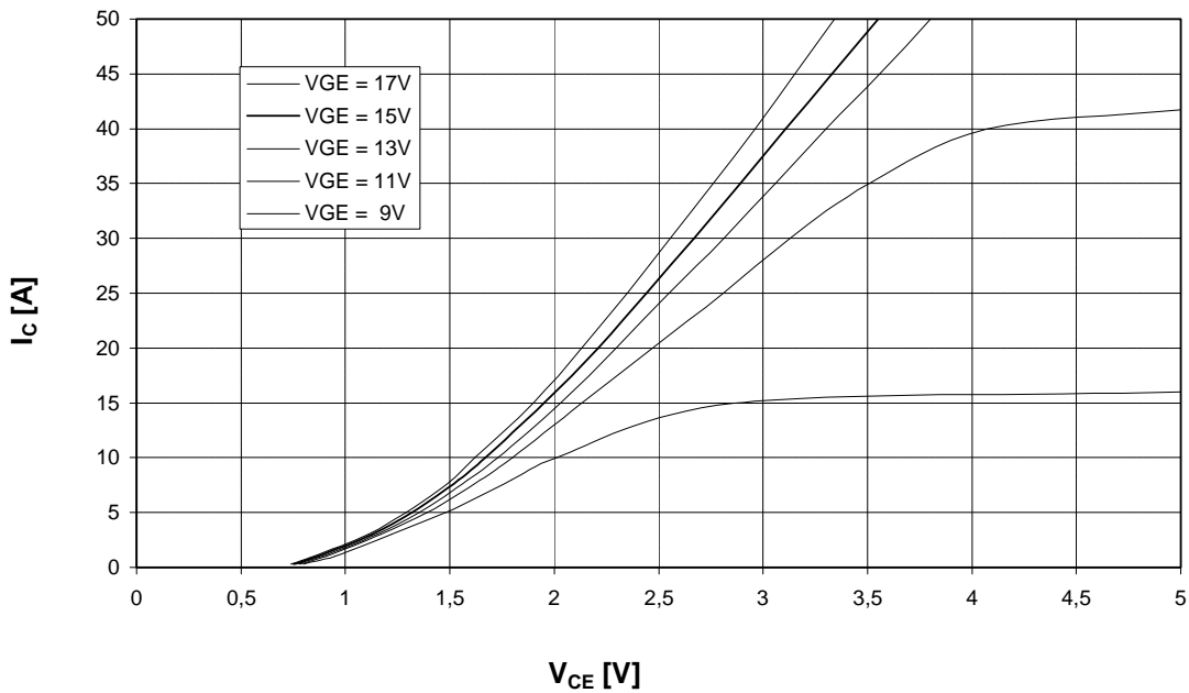
Output characteristic Inverter (typical)
