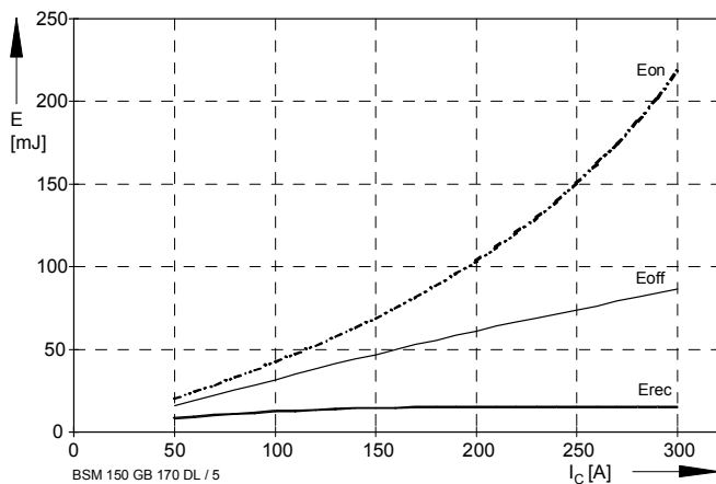
Bild / Fig. 5 Schaltverluste (typisch) / Switching losses (typical) E_{on} = f(I_C) , E_{off} = f(I_C) , E_{rec} = f(I_C) R_{gon} = R_{goff} = 10\Omega , V_{CE} = 900V , T_j = 125°C
